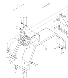
ETB-008086, Błotniki 20.8 R38
